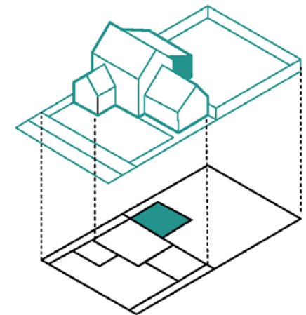
Figure 51: An acceptable example of a rear extension with a roof form and pitch which sits below the main ridge line of the original building.
